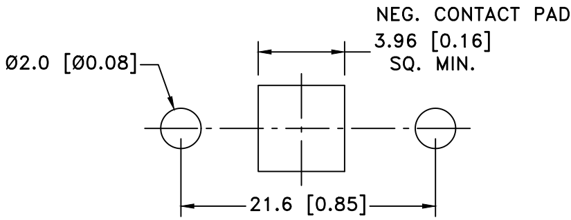
PCB LAYOUT
