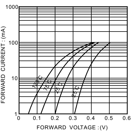
Fig. 1 Forward characteristics
